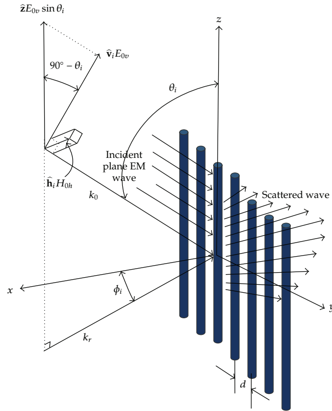
Figure 1: The schematic of the scattering by an infinite grating at oblique incidence.
