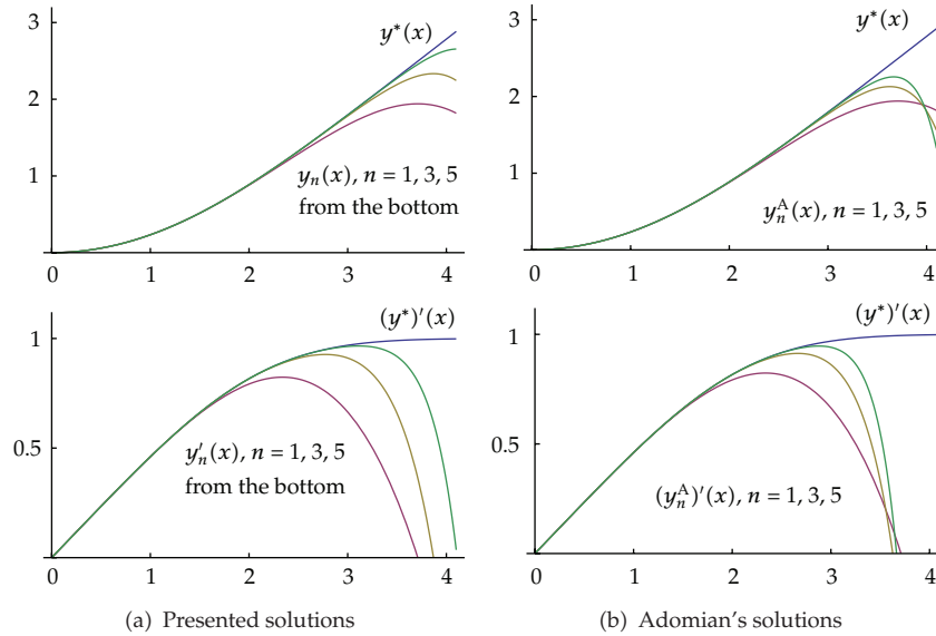
Figure 1: Graphs of the presented solutions y_n(x) and their derivatives y'_n(x) in (a) and those of Adomian's solutions y_n^A(x) and their derivatives (y_n^A)'(x) in (b).
