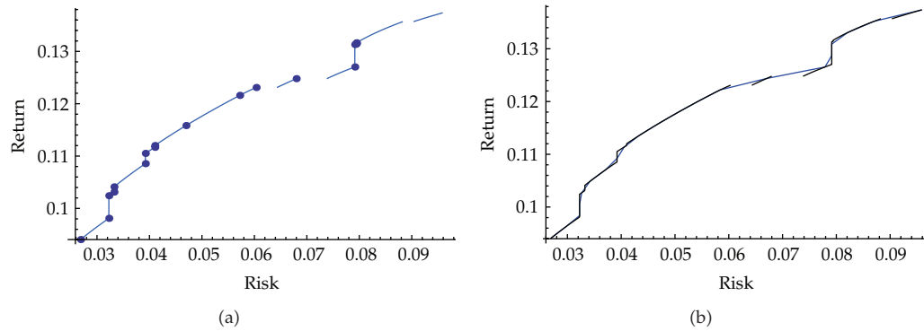
Figure 7: (a) The true efficient frontier. (b) The true frontier and a standard approximation.
