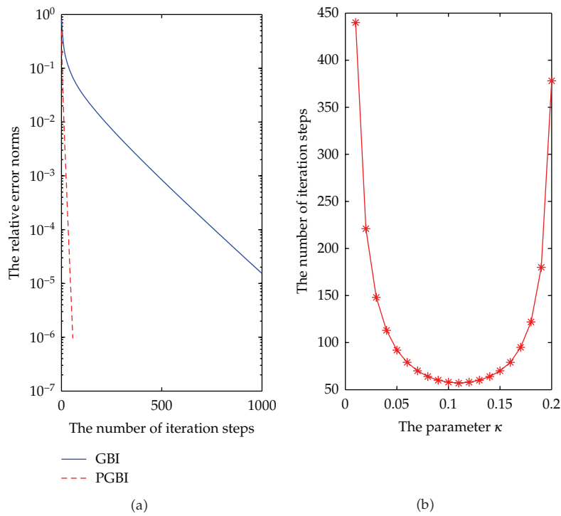
Figure 4: Comparison of convergence curves using GBI and PGBI (a); the influence of parameter \kappa on PGBI method (b).
