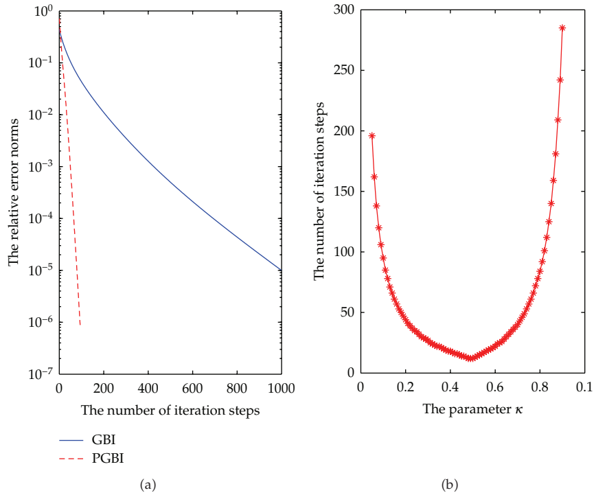
Figure 1: Comparison of convergence curves using GBI and PGBI (a); the influence of parameter \kappa on PGBI method (b).
