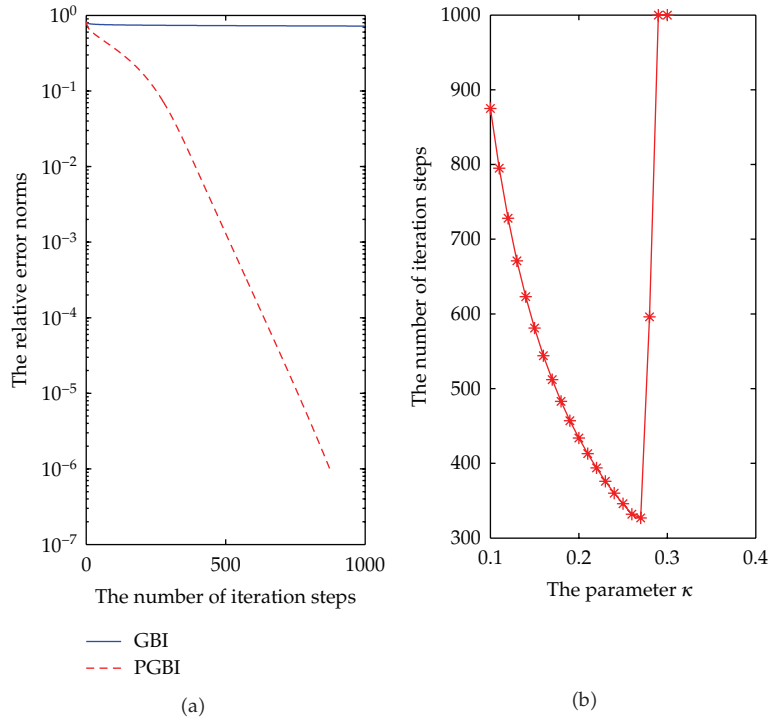
Figure 3: Comparison of convergence curves using GBI and PGBI (a); the influence of parameter \kappa on PGBI method (b).
