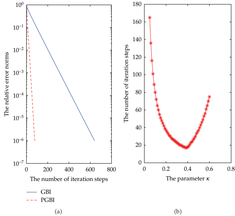
Figure 2: Comparison of convergence curves using GBI and PGBI (a); the influence of parameter \kappa on PGBI method (b).
