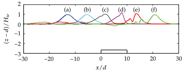
Figure 2: Transformation of a solitary wave travelling over a submerged breakwater with n = 0.2 and D_{50} = 0.05 m at different time levels: (a) t(g/d)^{0.5} = 35 , (b) t(g/d)^{0.5} = 42 , (c) t(g/d)^{0.5} = 49 , (d) t(g/d)^{0.5} = 56 , (e) t(g/d)^{0.5} = 63 , and (f) t(g/d)^{0.5} = 70 .
