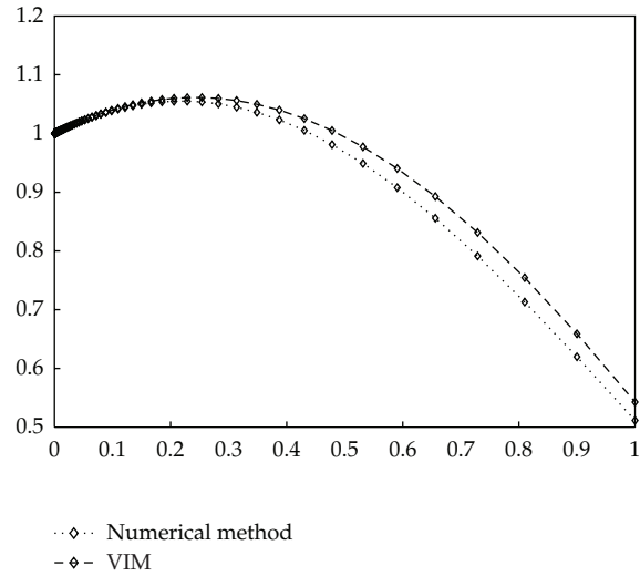
Figure 1: Time response for x^{\Delta\Delta} + (0.1 + 0.1x)x^{\Delta} + x + x^2 = 0 with 3 iterations.
