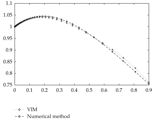
Figure 3: Time response for x^{\Delta\Delta} + (2.5 + 0.1x)x^{\Delta} + x + x^2 = 0 with 3 iterations.
