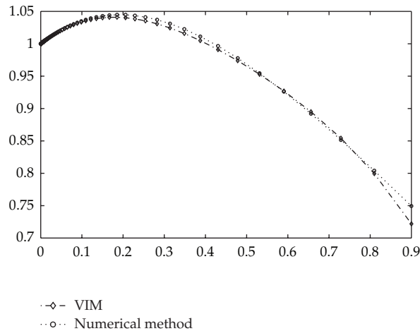
Figure 2: Time response for x^{\Delta\Delta} + (0.1 + 2.5x)x^{\Delta} + x + x^2 = 0 with 3 iterations.
