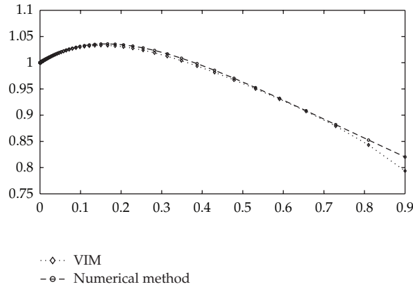
Figure 4: Time response for x^{\Delta\Delta} + (2.5 + 2.5x)x^{\Delta} + x + x^2 = 0 with 7 iterations.
