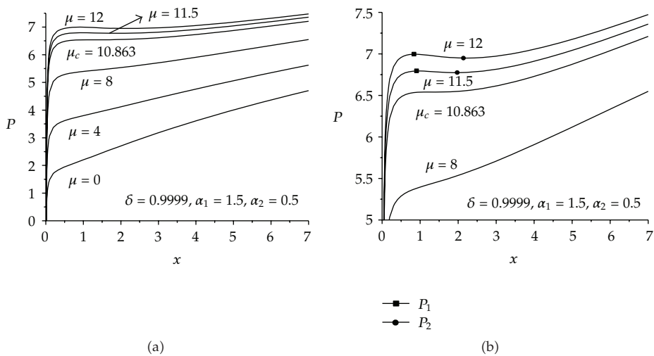
Figure 3: Curves of P \sim x for \alpha_1 > 1, 0 < \alpha_2 < 1 .
