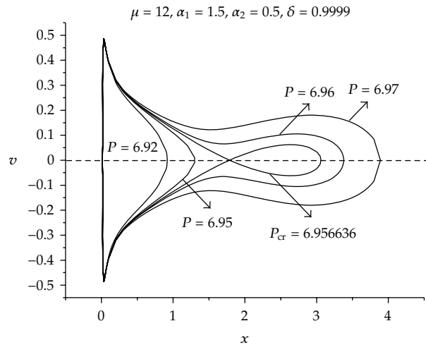
Figure 5: Phase diagrams for different values of P and for \mu = 12 , \alpha_1 = 1.5 , \alpha_2 = 0.5 , and \delta = 0.9999 .
