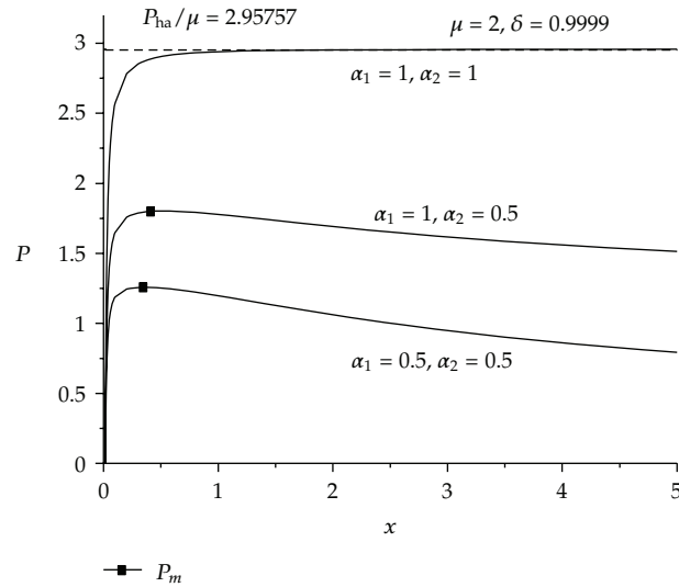
Figure 1: Curves of P \sim x for 0 < \alpha_1, \alpha_2 \leq 1 .
