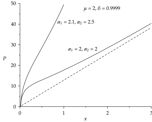
Figure 2: Curves of P \sim x for \alpha_1, \alpha_2 > 1 .
