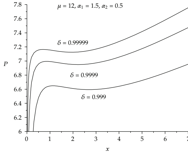
Figure 4: Curves of P \sim x for different values of \delta .
