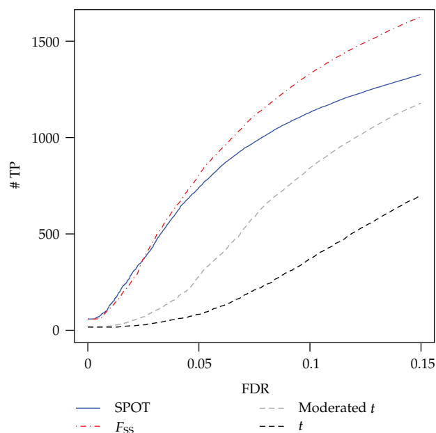
Figure 3: Simulation study III: plots of number of true positives (# TP) versus false discovery rate (FDR) from analyses using SPOT, moderated t , and F_{SS} methods.
