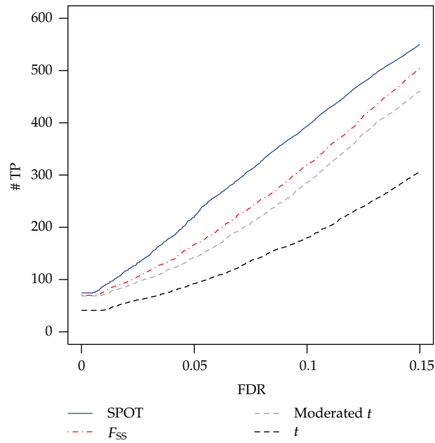
(a) Simulation I, setting 1
