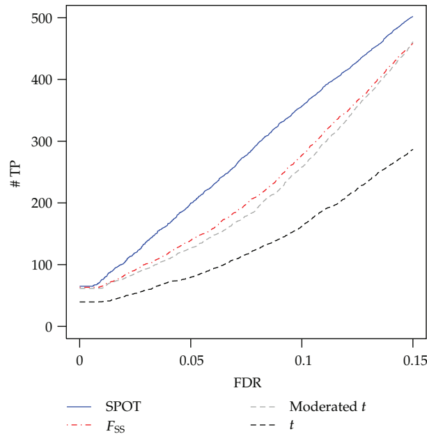
Figure 2: Simulation study II: plots of number of true positives (# TP) versus false discovery rate (FDR) from analyses using SPOT, moderated t , and F_{SS} methods.
