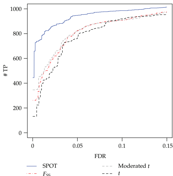
Figure 4: Golden spike data: plots of number of true positive (TP) genes versus false discovery rate (FDR) from analysis using SPOT, moderated t , and F_{SS} tests.
