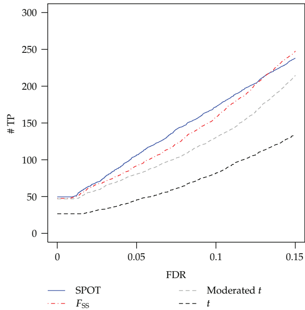
(b) Simulation I, setting 2
