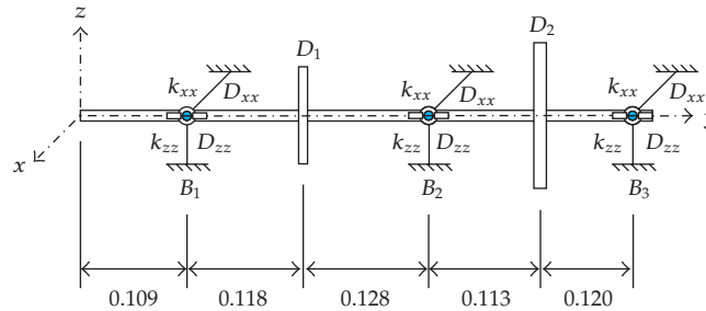
Figure 2: Rotor model.
