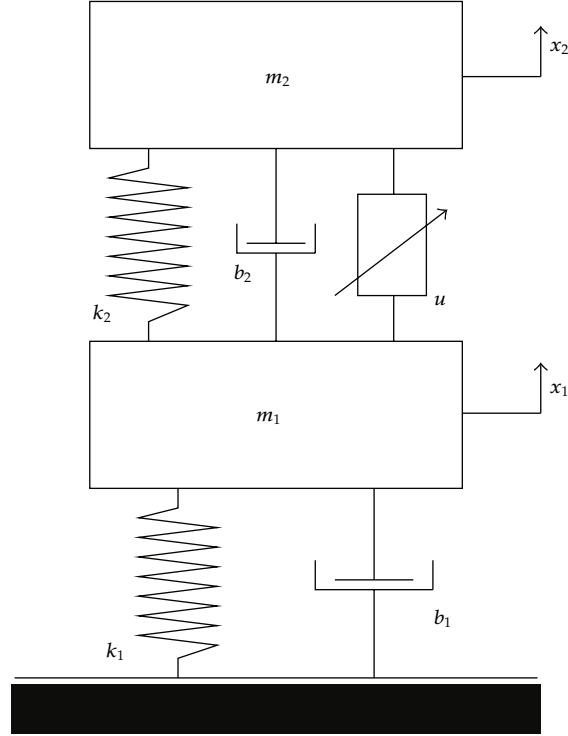
Figure 8: Mechanical vibration.
