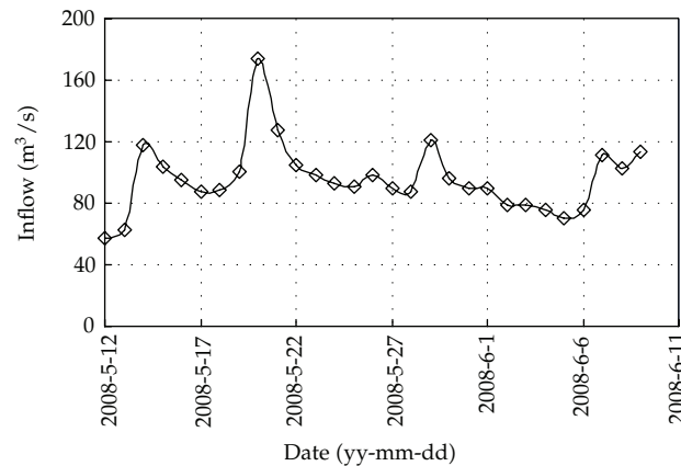
Figure 11: Results of monitoring the water inflow to the Tangjiashan landslide-dammed lake upstream.
