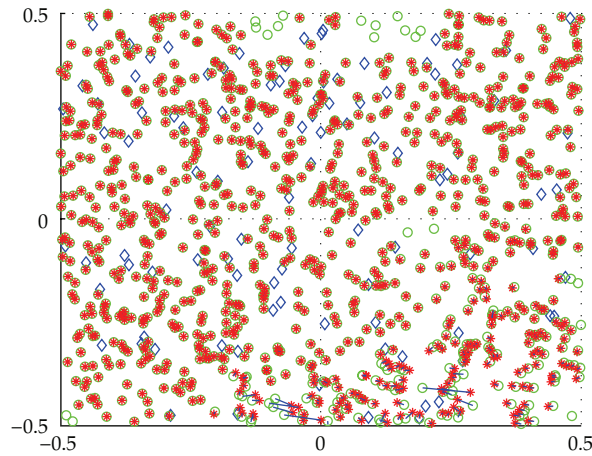
Figure 2: Graphical display of a sensor network with n = 1000 , m = 100 , rd = 0.06 , nf = 0.001 . The (blue) diamonds refer to the positions of the anchors; the (green) circles to the original locations of the unknown sensors; the (red) asterisks to their estimated positions by BU. The discrepancies between the original and the estimated points are indicated by the solid lines. RMSD = 5.9e-3 .
