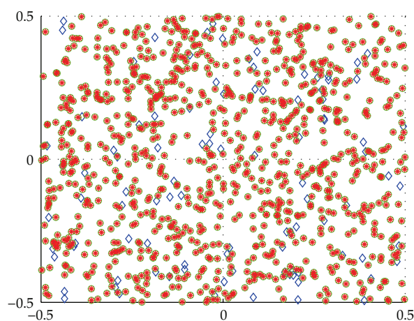
Figure 1: A network determined by the geometric buildup algorithm. n = 1000 , m = 100 , rd = 0.1 , nf = 0 . The (blue) diamonds refer to the positions of the anchors; the (green) circles to the original locations of the unknown sensors; the (red) asterisks to their estimated positions from the geometric buildup algorithm.
