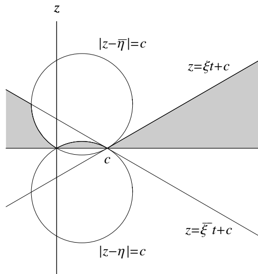
Figure 1: The shaded region, where t is a real parameter, \xi = c + i\sqrt{3}c/3 , and \eta = c/2 - i\sqrt{3}c/2 , represents the condition on a and b , with c being fixed, such that Newton's inequalities hold.
