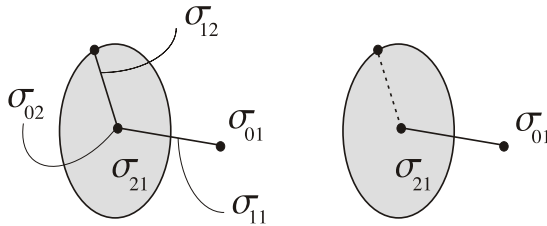
Figure 2: Firm and not firm triplets
