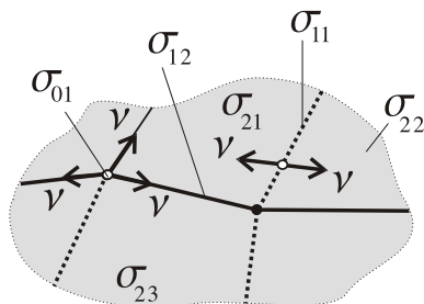
Figure 1: An example of stratified set
