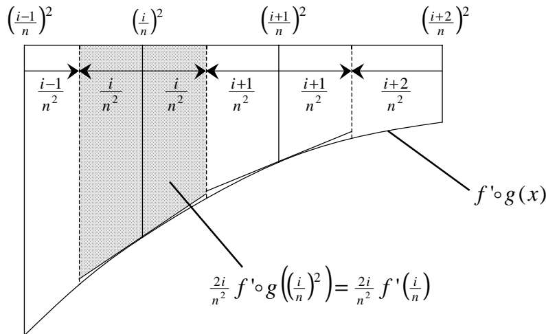
Figure 1: A trapezium estimate for the integral of the concave function f' \circ g where g(x) = x^{\frac{1}{2}} .
