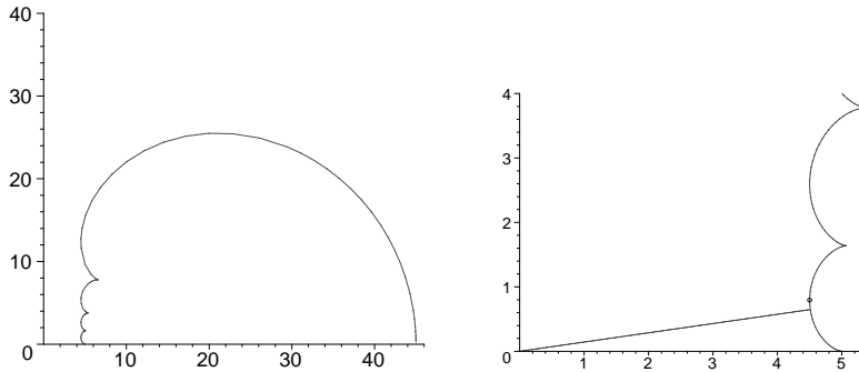
Figure 1: Graph of z_0 .
