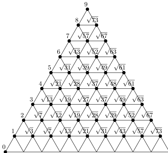
Figure 2: Triangular lattice points \Lambda_1 \cup \{0\} along with their distances from the origin ( i \leq 9 ).
