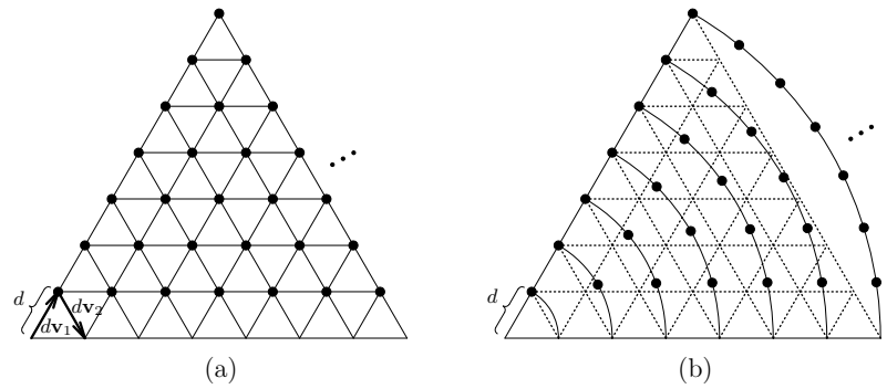
Figure 1: Illustration of two point sets along with related parameters: (a) \Lambda_d and (b) \Omega_d .
