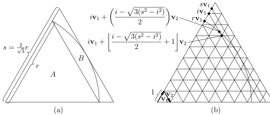
Figure 3: Illustration of (a) regions A and B and constants r and s , and (b) points related to B .
