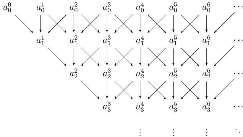
Figure 1: Construction of the trinomial transform triangle \mathcal{T}
