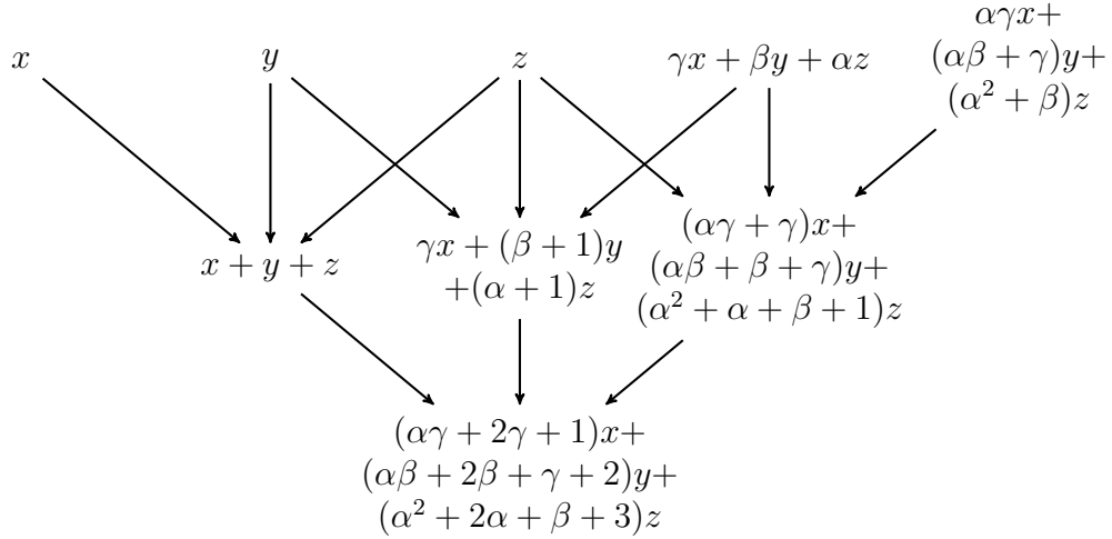
Figure 4: A part of the growing of \mathcal{T}
