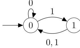
Figure 1: The 2-DFAO generating the period-doubling sequence \mathbf{d} .
