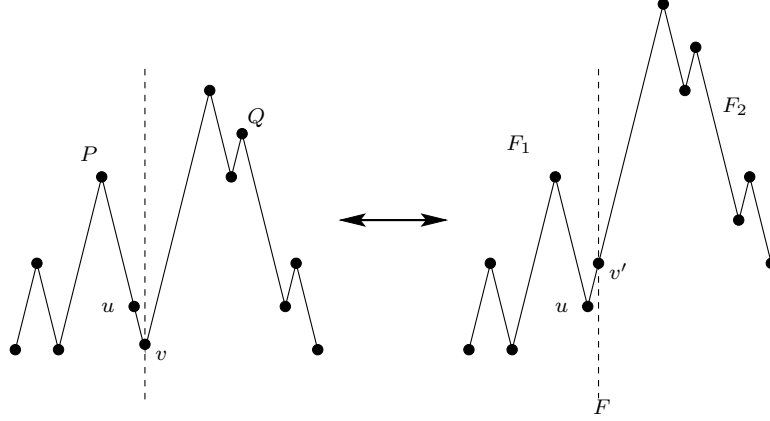
Figure 1: First step of the bijection
