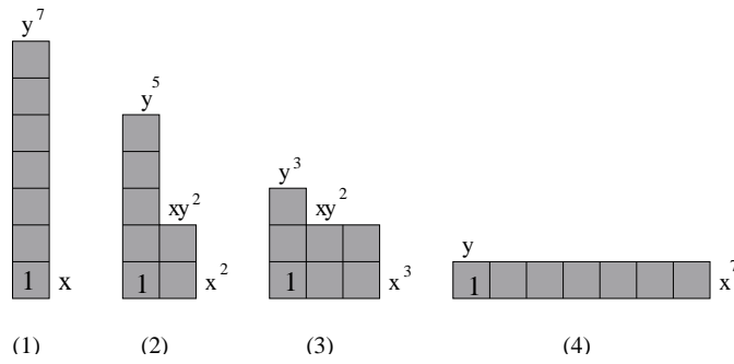
FIGURE 4.4. G -cluster Y(Z_p)
