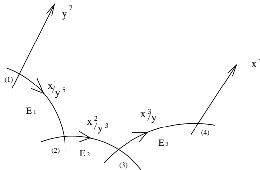
FIGURE 4.2. Configuration of \tilde{X}
