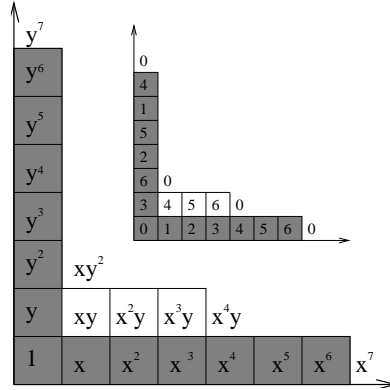
FIGURE 4.3. G -basis B(G) and the characters
