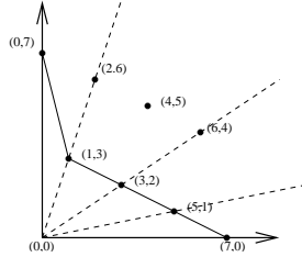
FIGURE 4.1. Toric resolution of \mathbb{C}^2/G
