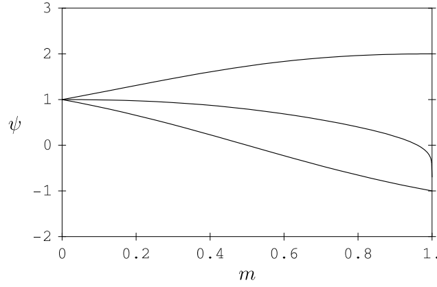
Figure 1. The upper, middle and lower curves are \psi = \psi_1(m) , \psi = \psi_2(m) and \psi = \psi_3(m) , respectively.
