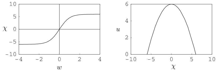
Figure 15. \beta = -4 so that \psi = -1 and v = 0 . The solution for u is a solitary wave with compact support.
