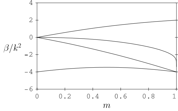
Figure 2. From the top, the curves correspond to \beta = \beta_1(m) , \beta = \beta_2(m) , \beta = \beta_3(m) and \beta = \beta_4(m) , respectively.
