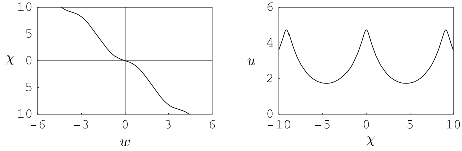
Figure 3. \beta = 2.1 > \beta_1 so that \psi > \psi_1 . The wave profile comprises periodic smooth humps.
