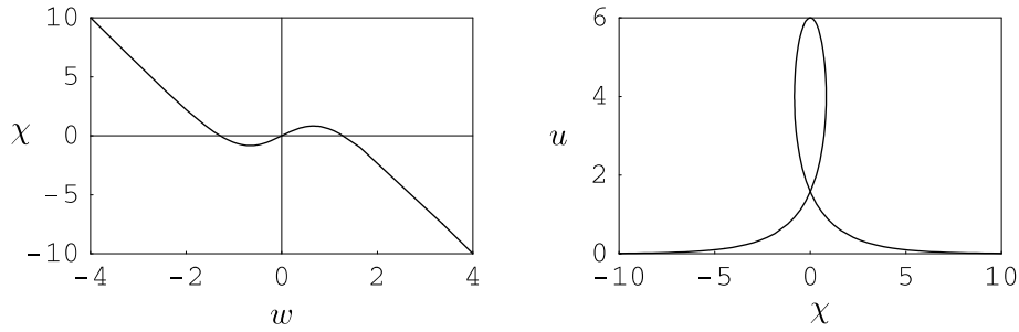
Figure 13. \beta = 0 so that -1 < \psi < 2 and v > 0 . The wave profile comprises a solitary loop.
