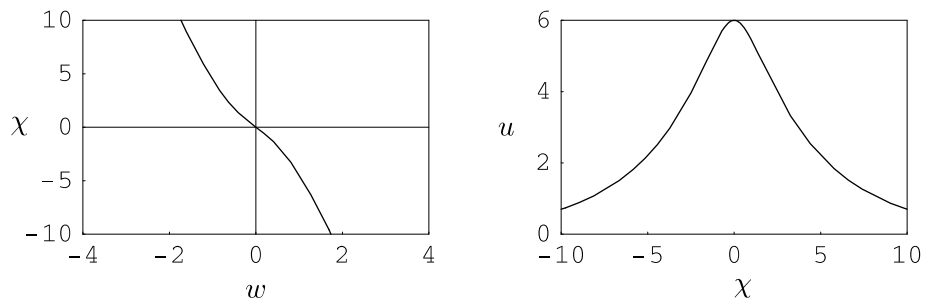
Figure 11. \beta = 5 so that \psi > 2 and v > 0 . The wave profile is a solitary smooth hump.
