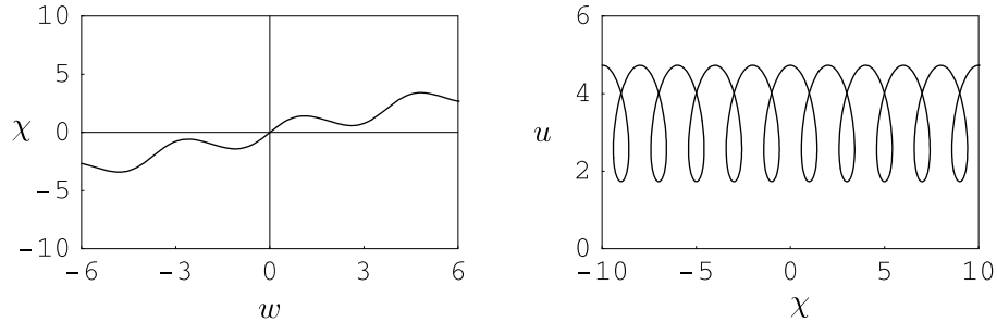
Figure 6. \beta = -0.9 so that \beta_3 < \beta < \beta_2 , i.e. \psi_3 < \psi < \psi_2 . The wave profile comprises periodic inverted loops.
