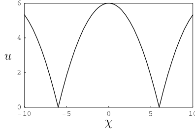
Figure 16. A composite solution corresponding to Fig. 15. The wave profile comprises periodic corner waves.
