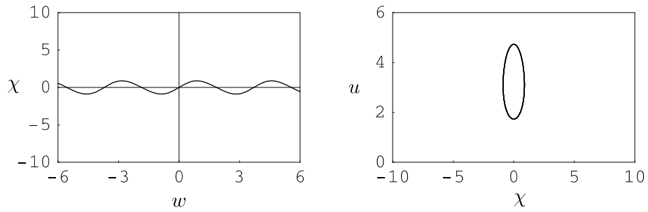
Figure 9. \beta = \beta_2 so that \psi = \psi_2 . The solution for u is a closed curve.
