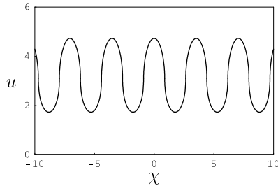
Figure 10. A composite solution corresponding to Fig. 9. The wave profile comprises periodic bells.
