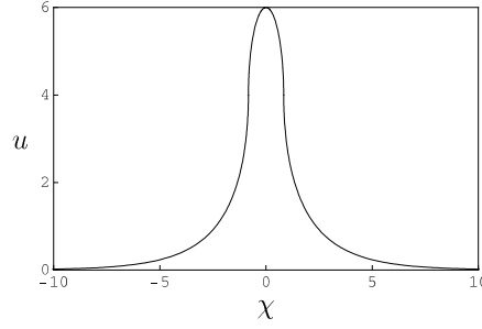
Figure 17. A single-valued composite solution corresponding to Fig. 13.
