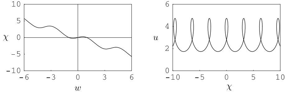
Figure 5. \beta = 0.5 so that \beta_2 < \beta < \beta_1 , i.e. \psi_2 < \psi < \psi_1 . The wave profile comprises periodic loops.
