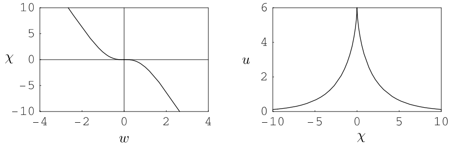
Figure 12. \beta = 2 so that \psi = 2 and v > 0 . The wave profile is a solitary cuspon.
