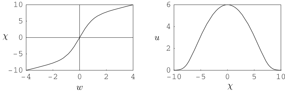
Figure 14. \beta = -5 so that \psi < -1 and v < 0 . The wave profile is a solitary smooth hump.
