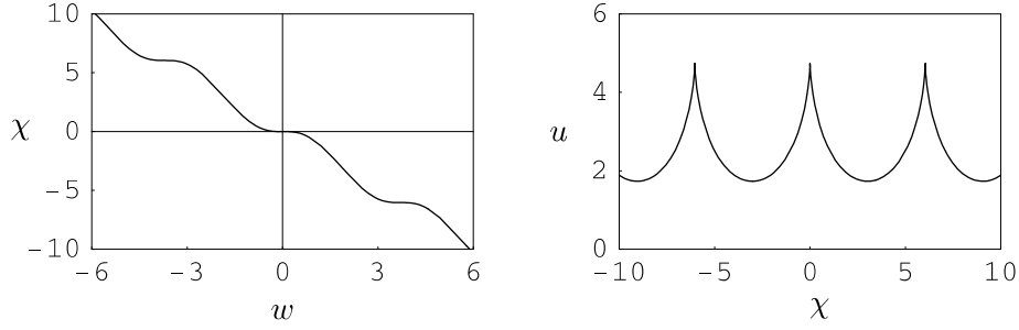
Figure 4. \beta = \beta_1 so that \psi = \psi_1 . The wave profile comprises periodic cusps.
