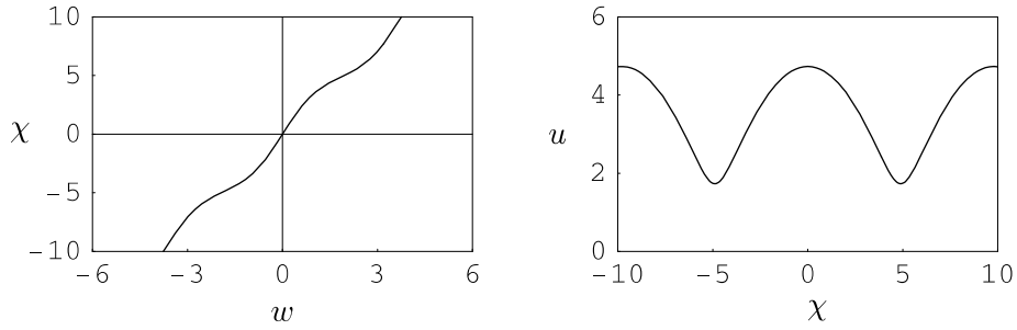
Figure 8. \beta = -3 < \beta_3 so that \psi < \psi_3 . The wave profile comprises periodic smooth humps.
