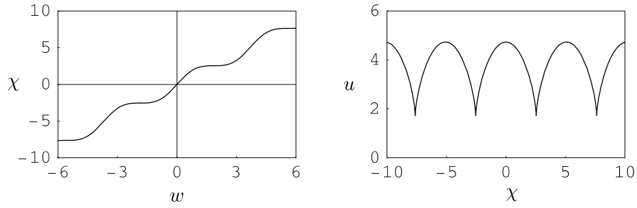
Figure 7. \beta = \beta_3 so that \psi = \psi_3 . The wave profile comprises periodic inverted cusps.
