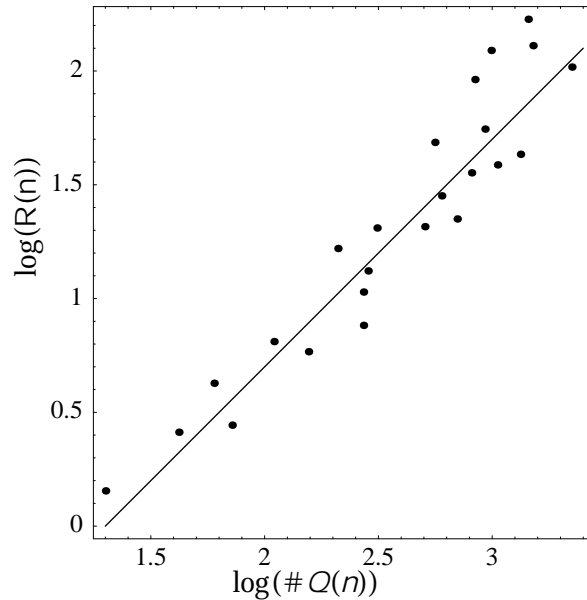
Figure 6: This plot shows the relationship between the expected rank and the degree of the cover. The line shown is y = x - 1.3 .
