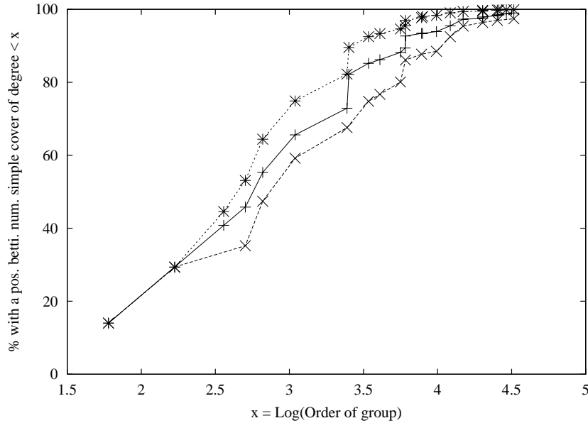
Figure 5: The top line plots (\log(\# Q(n)); V^0(n)) , the middle line (\log(\# Q(n)); V(n)) (as in Figure 4), and the lowest line plots only the groups of the form L_2(q) .
