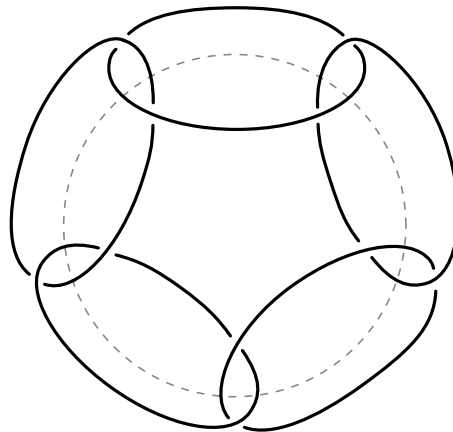
Figure 2: The minimally-twisted 5-chain link.
