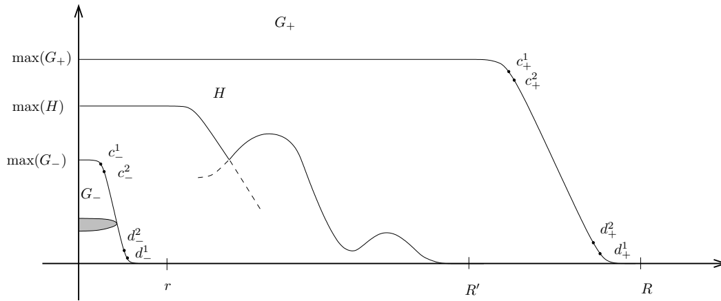
Figure 1: The functions G_+ and G_-
