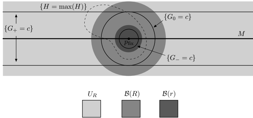
Figure 2: The supports of G_+ , G_0 and G_-
