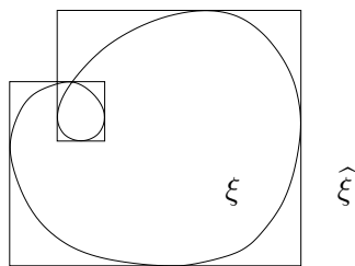
Figure 5: The curves \xi and \widehat{\xi}
