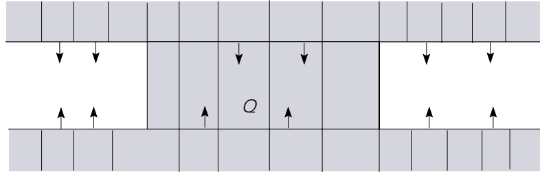
Figure 5: Opposed orientations on @_h Q
