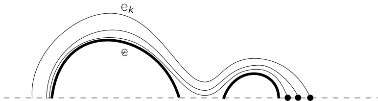
Figure 2: Non-Hausdorff accumulation of f_{e_k} g_{k=1}^{-1} on leaves of \mathcal{L}_+^\theta
