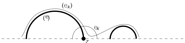
Figure 3: (e_k) crosses the geodesic e_k twice
