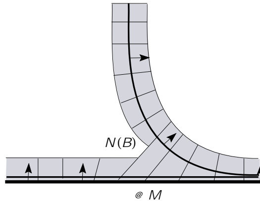
Figure 4: The normal neighborhood N(B) near @ M
