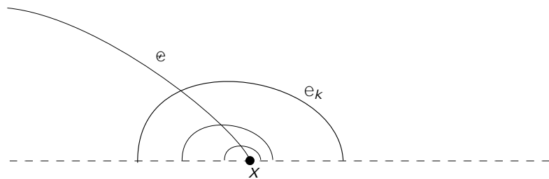
Figure 1: Each end of e limits to a point at infinity in \mathbb{E}^0
