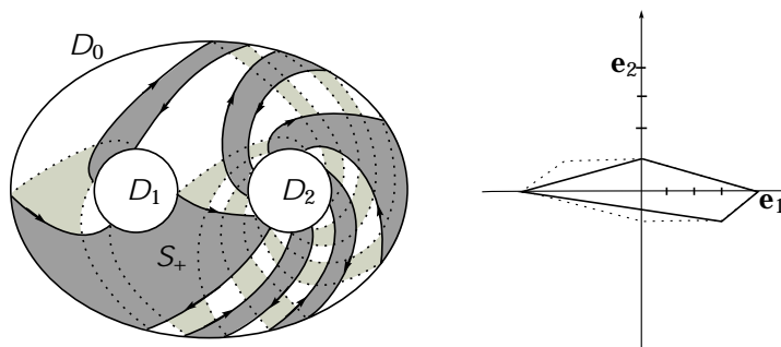
Figure 19: Example in which fD_1; D_2g does not work as Markov partition
