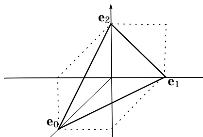
Figure 11: Foliation cones for (2;2;2)
