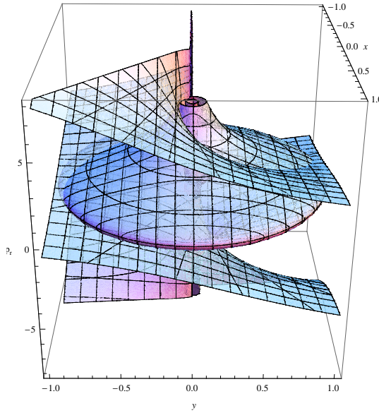
Figure 1. The level sets of H (the central “bubble”) and of \mathcal{J}_+ (the helicoid-like surface) for L = 1, A = 2, \nu = 1/3, H = -1.95 and \arg(\mathcal{J}_+) = -0.9 .
