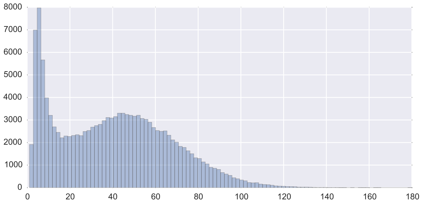
Subject 23780 tSNR inside the mask
