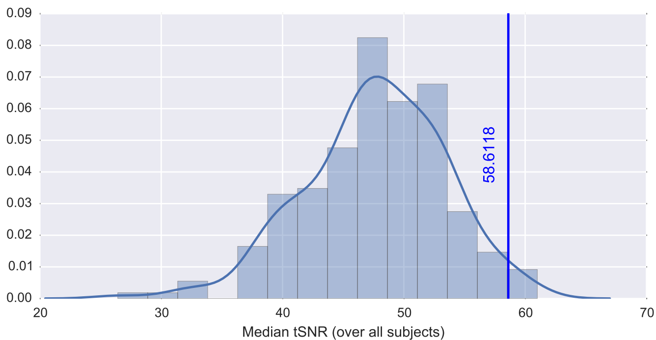
Subject 26782 tSNR inside the mask
