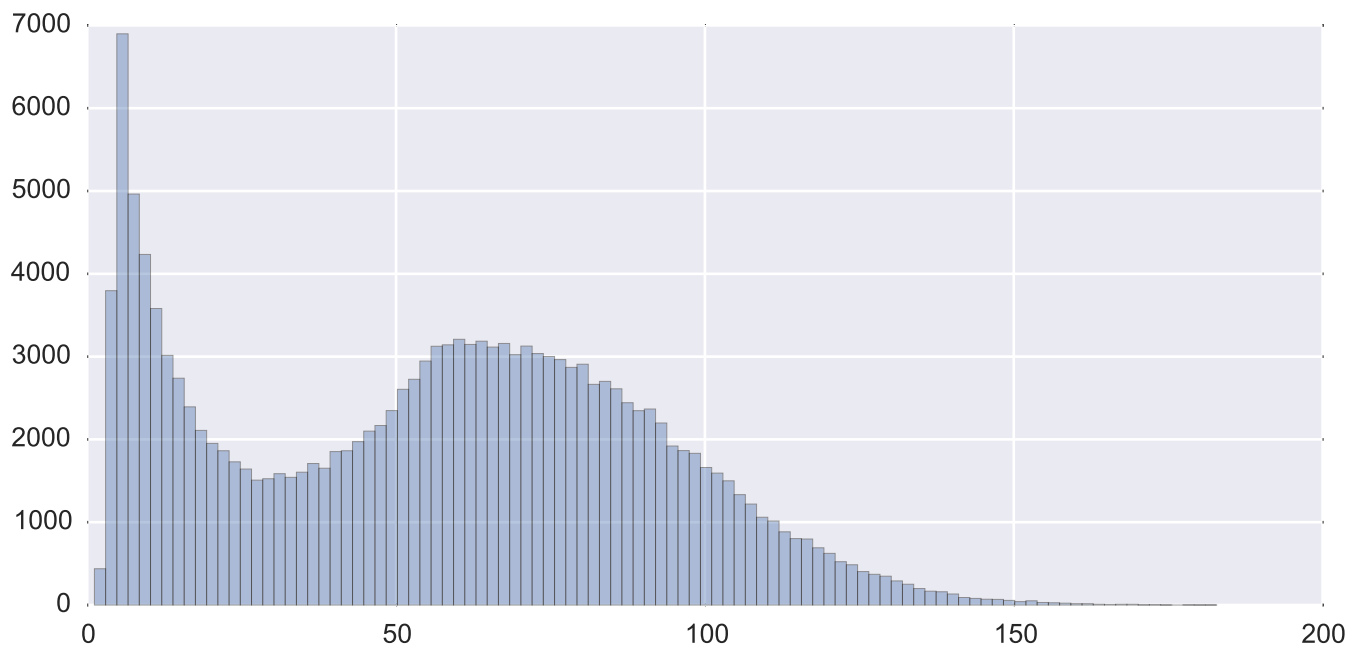
Subject 26782 tSNR inside the mask
