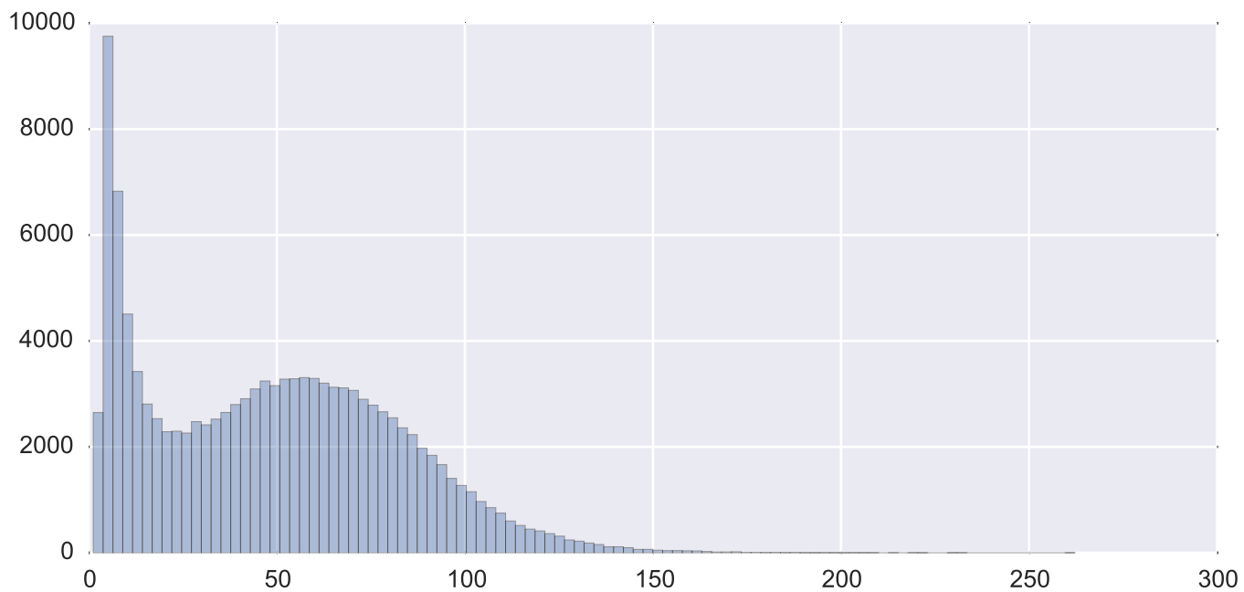
Subject 26856 tSNR inside the mask
