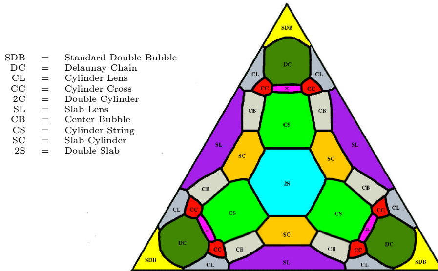
FIGURE 2. Phase portrait: volumes and corresponding double bubble. In the center both regions and the complement have one third of the total volume; along the edges, one volume is small; in the corners, two volumes are small.
