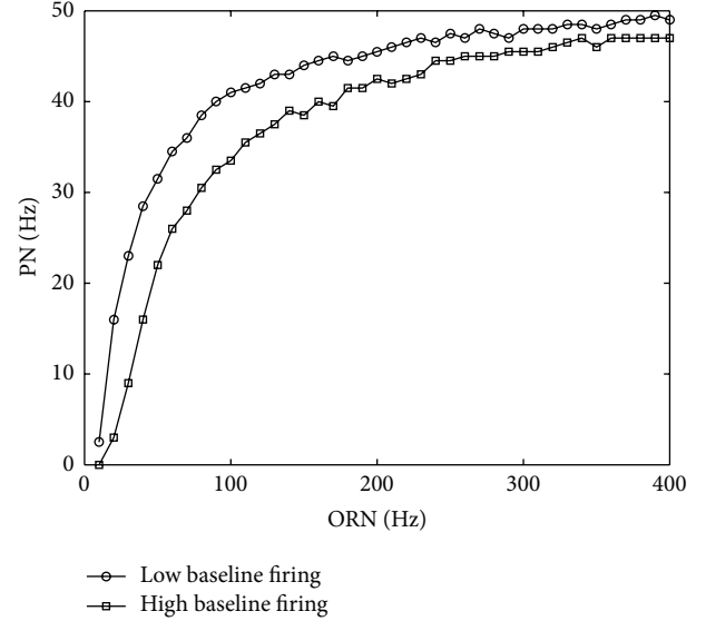
FIGURE 2: The ORN-PN response curve is modulated by the total activity of ORNs. In the low and high baseline cases, the firing rates of other ORNs are set to be 20 Hz and 30 Hz, respectively. Symbols denote the simulation results. The parameters are N^E = 49 ; K = 40 ; N^I = 20 ; w^{EE} = 10 nS; w^{EI} = 0.05 nS; w_i^I = 0.1 nS; \tau_D = 100 ms; \tau_E = 5 ms; \tau_I = 100 ms; C^E = 800 pF; C^I = 800 pF; g_L = 25 nS; E_L = -70 mV; E_E = 0 mV; v_{th} = -50 mV; v_{reset} = -70 mV; a = 0.3 ; \alpha^I = 3.76 ; \beta = 5.65 ; b = aN^I \alpha^I \beta \tau_I w^I .
