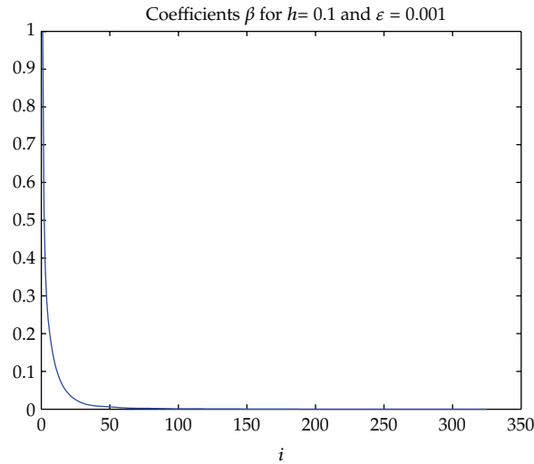
Figure 4: Coefficients \beta for \epsilon = 0.001 .
