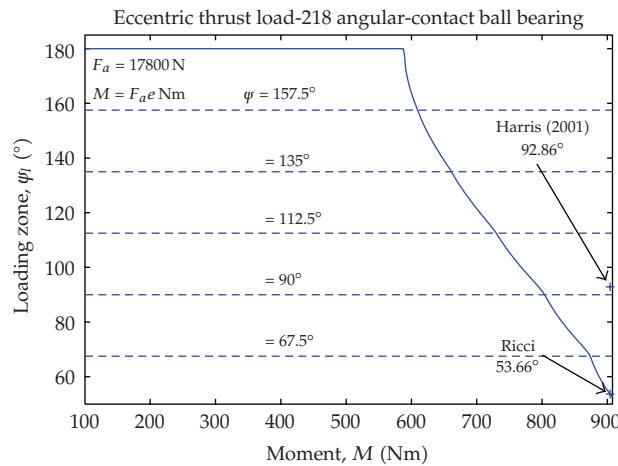
Figure 13: Loading zone, \psi_t , for 17,800 N thrust load, as a function of the Moment, M .
