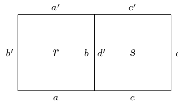
FIGURE 5. Definition M_1 .
