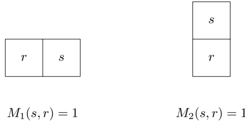
FIGURE 4. Definition of the transition matrices.
