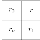
FIGURE 6. A word of shape (1, 1) .
