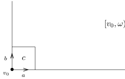
FIGURE 12. A sector representing \omega \in \Omega(c) .
