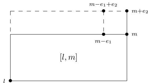
FIGURE 7. w(m + e_2) determines w on the rectangle [l, m + e_2] .
