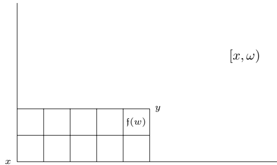
FIGURE 11. The rectangle R = \text{conv}(x, y) associated to a word w \in W_{(4,1)} , and the sector [x, \omega) representing a boundary point \omega \in \Omega(w) .
