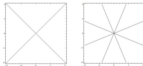
FIGURE 4. The zero level curves for \text{Re}(f_0) and \text{Re}(f_0^2) .
