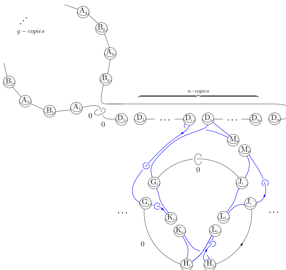
FIGURE 29. The LCF manifolds M_{g,n}^3 .
