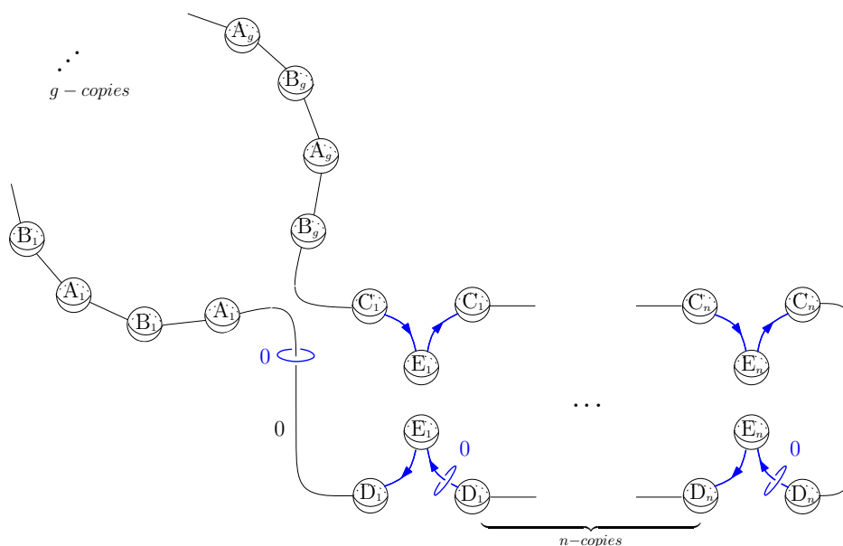
FIGURE 27. The LCF manifolds M_{g,n}^2 .
