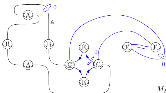
FIGURE 23. Maskit's 1/3 complex twist operation.
