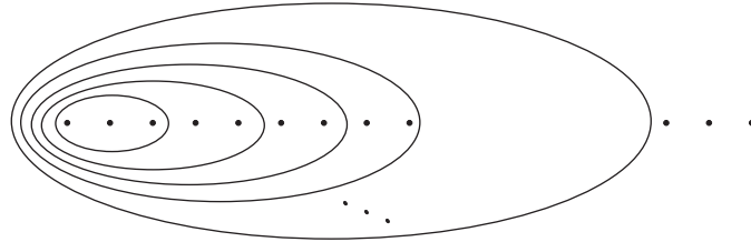
FIGURE 3. The projection of disjoint symmetric separating curves is S_{0,0,2g+2} when g = n + 1 and b = 0 .
