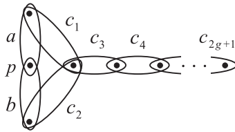
FIGURE 13. The curves needed for the proof of Lemma 5.3.
