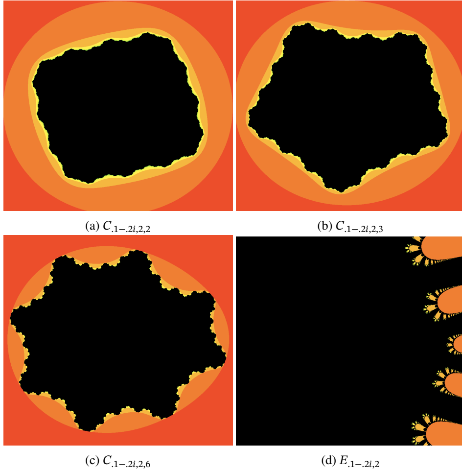
FIGURE 7. Julia and Fatou sets for C_{a,m,d} and E_{a,m} when a = 0.1 - 0.2i and m = 2 .
