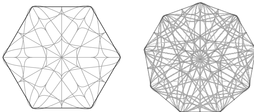
FIGURE 27. Portions of the flow graphs of veering branched surfaces constructed on T^1S \setminus \vec{c} projected onto n -gon complementary regions of c , for n = 6 (left) and n = 9 (right).
