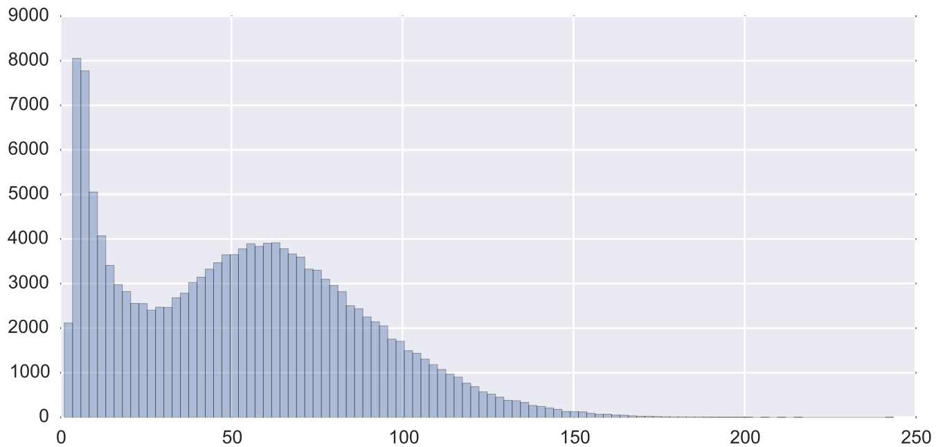
Subject 23428 tSNR inside the mask
