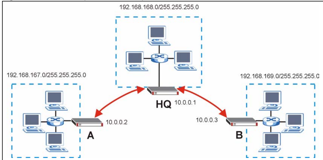
Figure 190 Hub-and-spoke VPN Example
